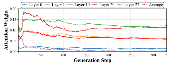
Figure 7: Dynamic attention during decoding. Consistent attention weights across generation steps indicate that the model continuously refers to structural priors.
