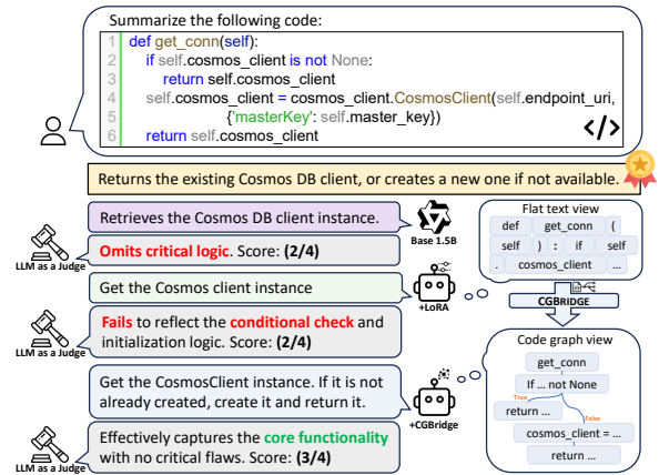
Figure 8: Case study on capturing control flow logic. While Base and LoRA models miss the critical lazy-initialization check ( if... is not None ), CGBRIDGE accurately captures this conditional logic.
